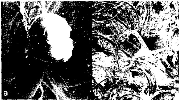
Fig. 1. Electron micrographs of the burr. (a) the closure side showing the mushroom-like structures (magnification x300). The diameters of the heads of the mushrooms range between 0.3 and 0.6 mm. (b) the loop side showing multiple slings (magnification x 150).
